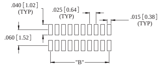
SUGGESTED PAD LAYOUT
