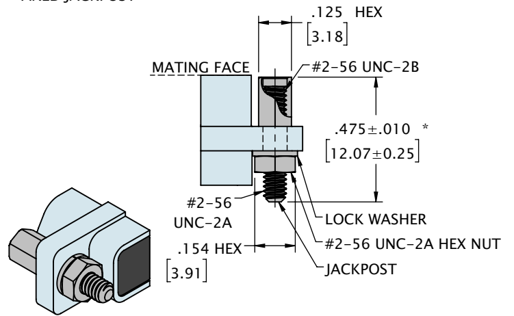
HARDWARE OPTION 01 - FIXED JACKPOST
