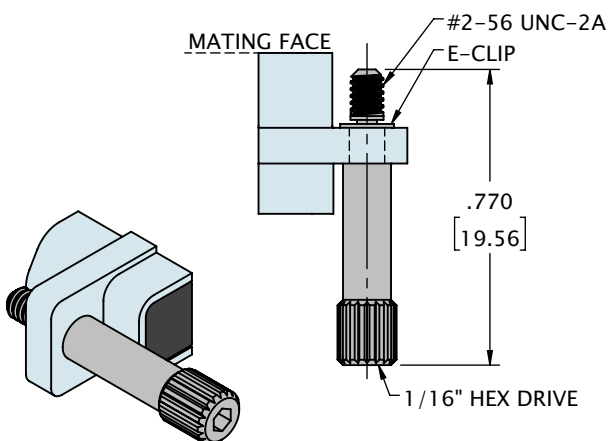
HARDWARE OPTION 04 - JACKSCREW, LONG LENGTH W/ HEX DRIVE
